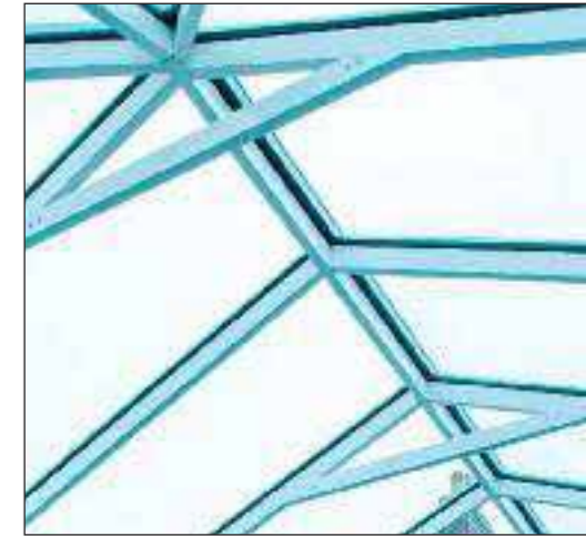
Roofs 3.8m-5m wide - slim tie bar
